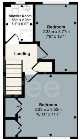
First Floor Approx 30 sq m / 324 sq ft
